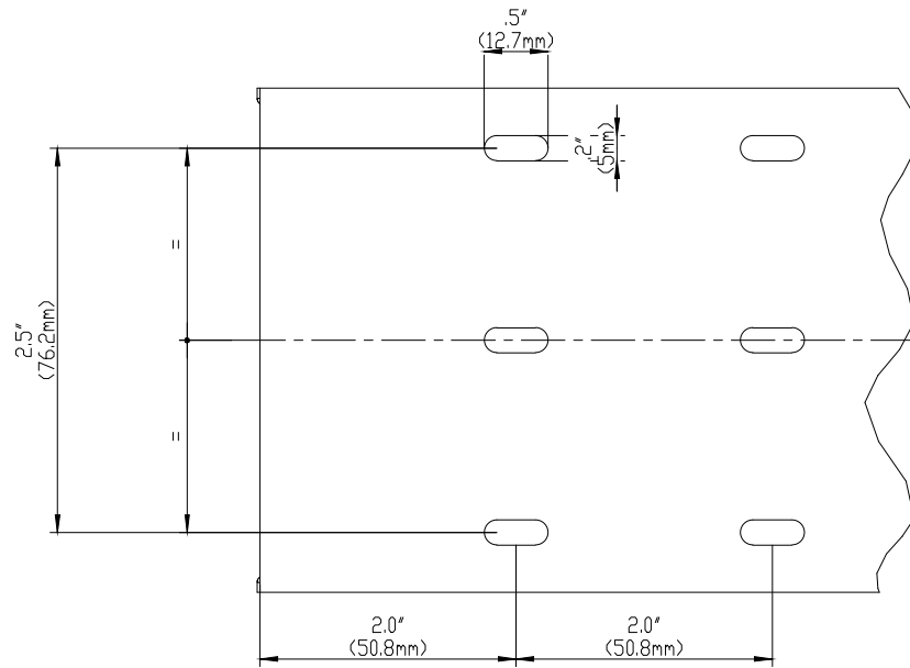
FRONT SECTION
