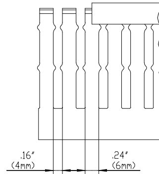
SIDE SECTION
