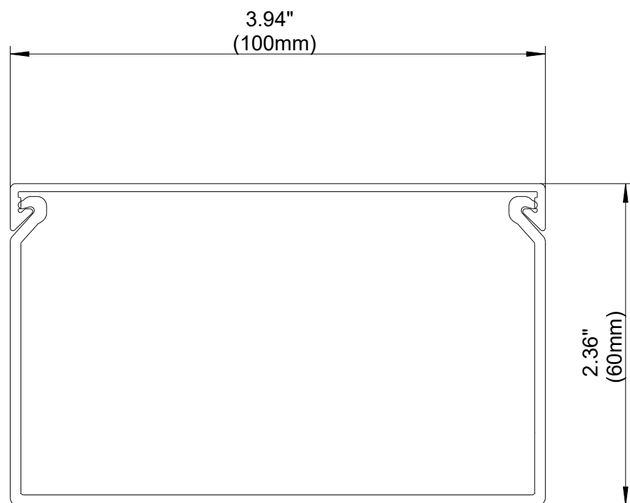
FRONT SECTION
