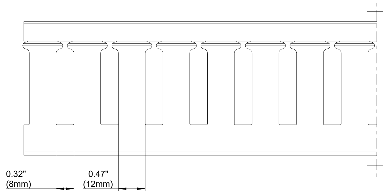
SIDE SECTION
