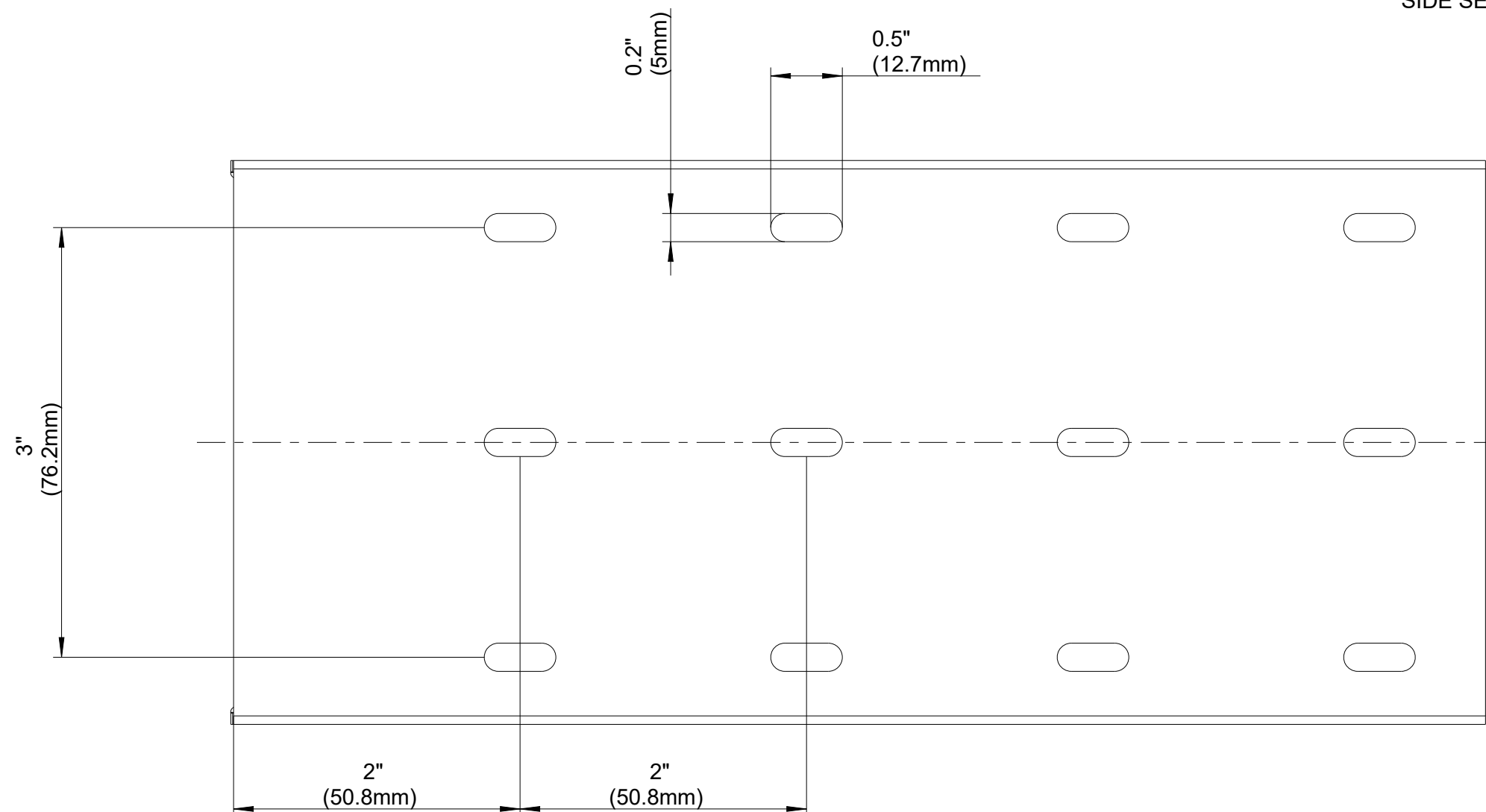
BASE PERFORATION
