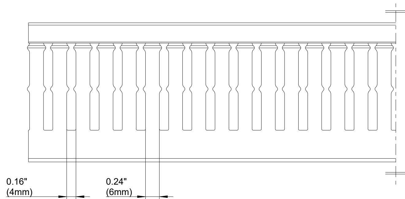
SIDE SECTION
