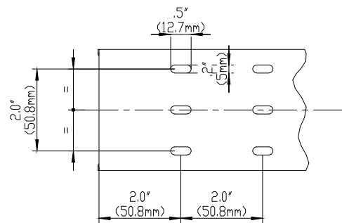
BASE PERFORATION
