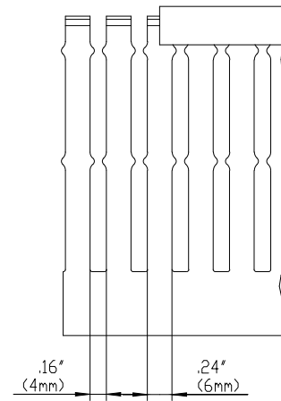
SIDE SECTION
