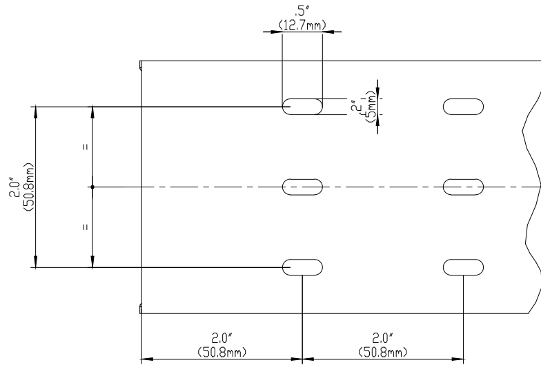
BASE PERFORATION
