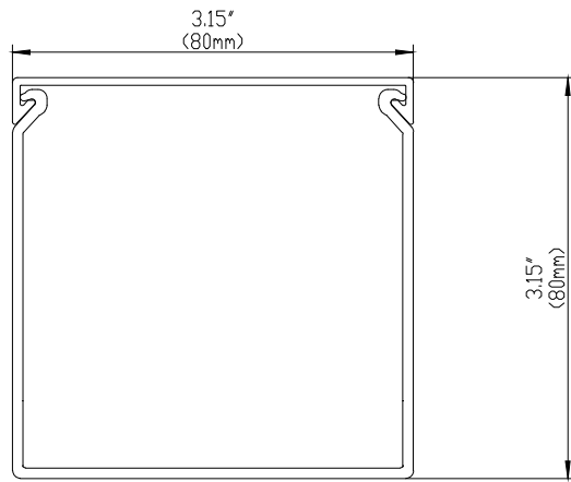
FRONT SECTION
