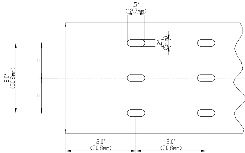
BASE PERFORATION
