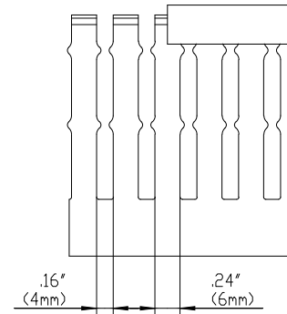
SIDE SECTION
