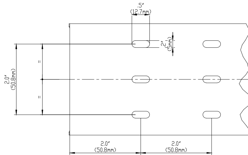
BASE PERFORATION
