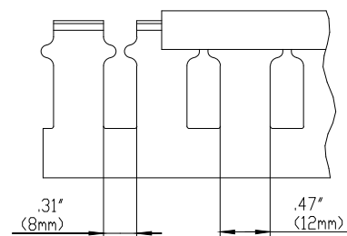
SIDE SECTION
