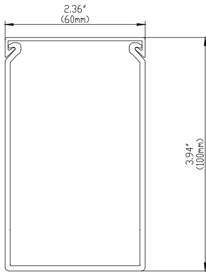
FRONT SECTION
