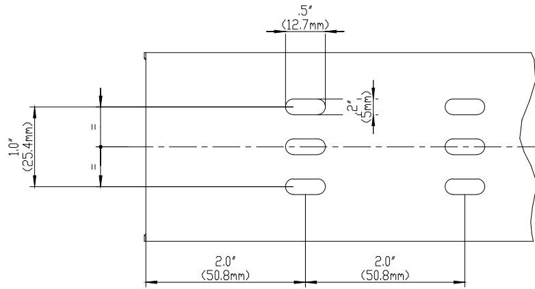
BASE PERFORATION
