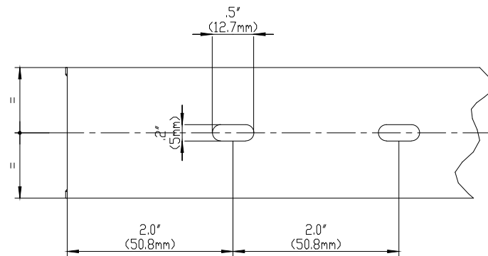
BASE PERFORATION
