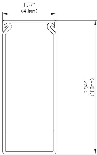
FRONT SECTION
