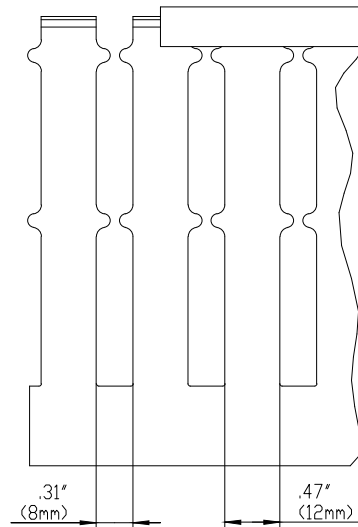
SIDE SECTION
