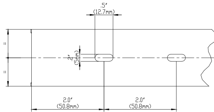
BASE PERFORATION
