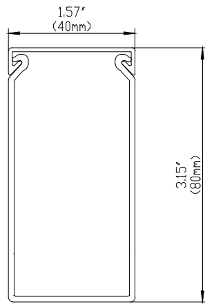
FRONT SECTION
