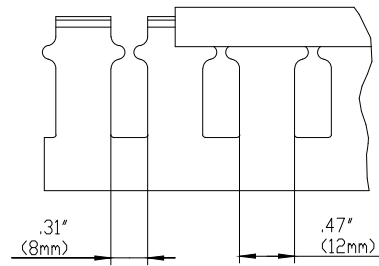
SIDE SECTION
