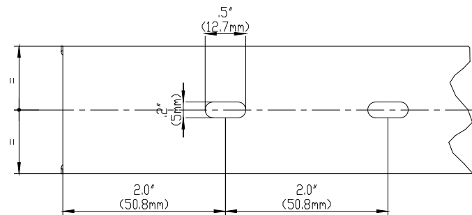
BASE PERFORATION
