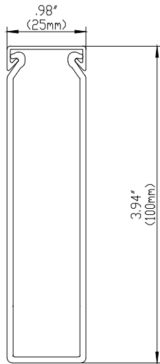
FRONT SECTION
