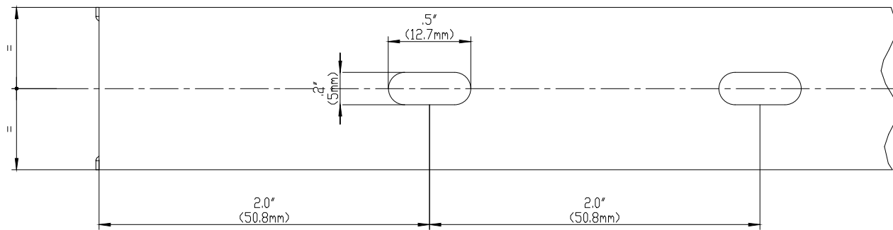
BASE PERFORATION
