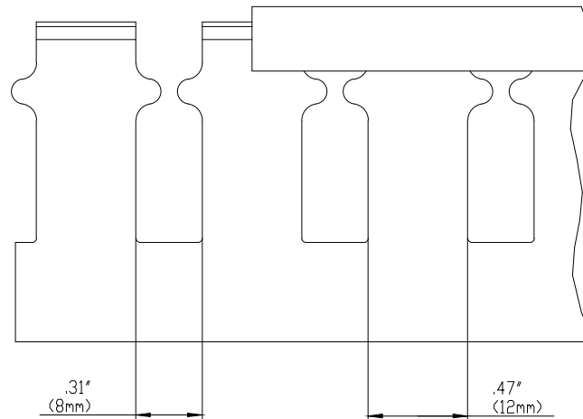
SIDE SECTION
