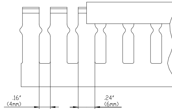
SIDE SECTION
