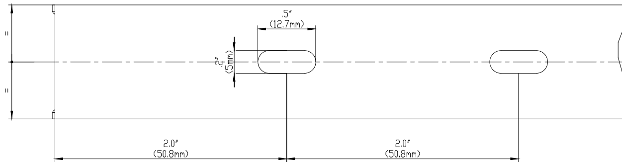
BASE PERFORATION
