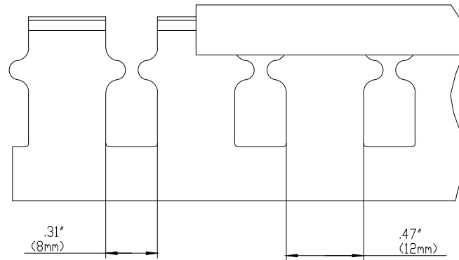
SIDE SECTION
