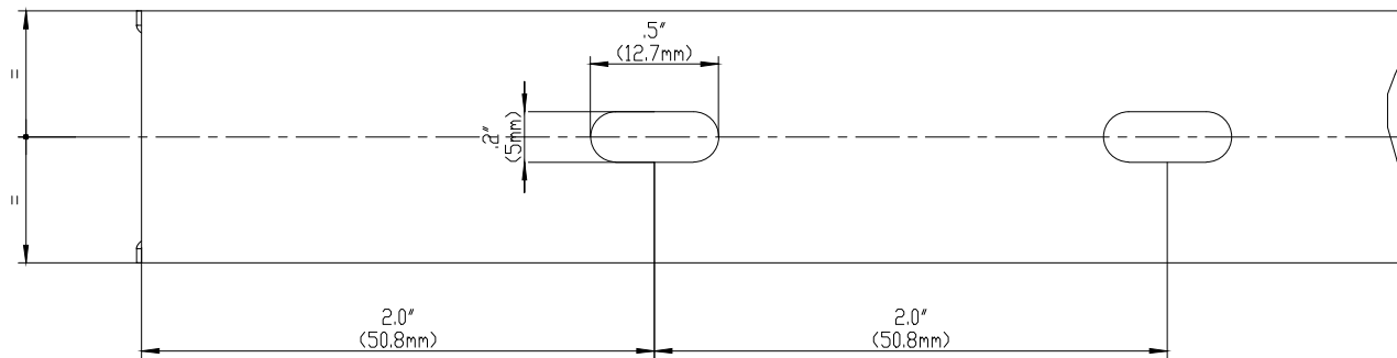
BASE PERFORATION
